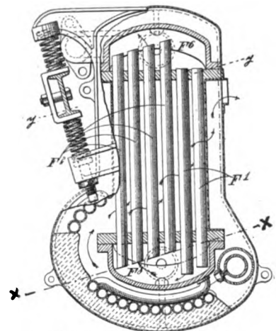
BARBER STEAM GENERATOR.
